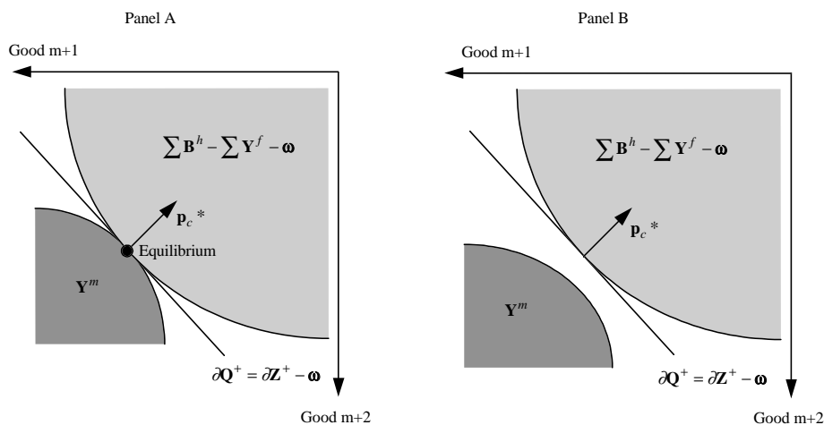
Figure 4.1: The boundary of \mathbf{Q}^+ separates \sum \mathbf{B}^h - \sum_{f \neq m} \mathbf{Y}^f - \boldsymbol{\omega} from \mathbf{Y}^m in an efficient equilibrium. The cross-section in Panel A holds the m monopoly goods equal to their equilibrium level \mathbf{y}_m^{m*} ; Panel B depicts another cross-section.
